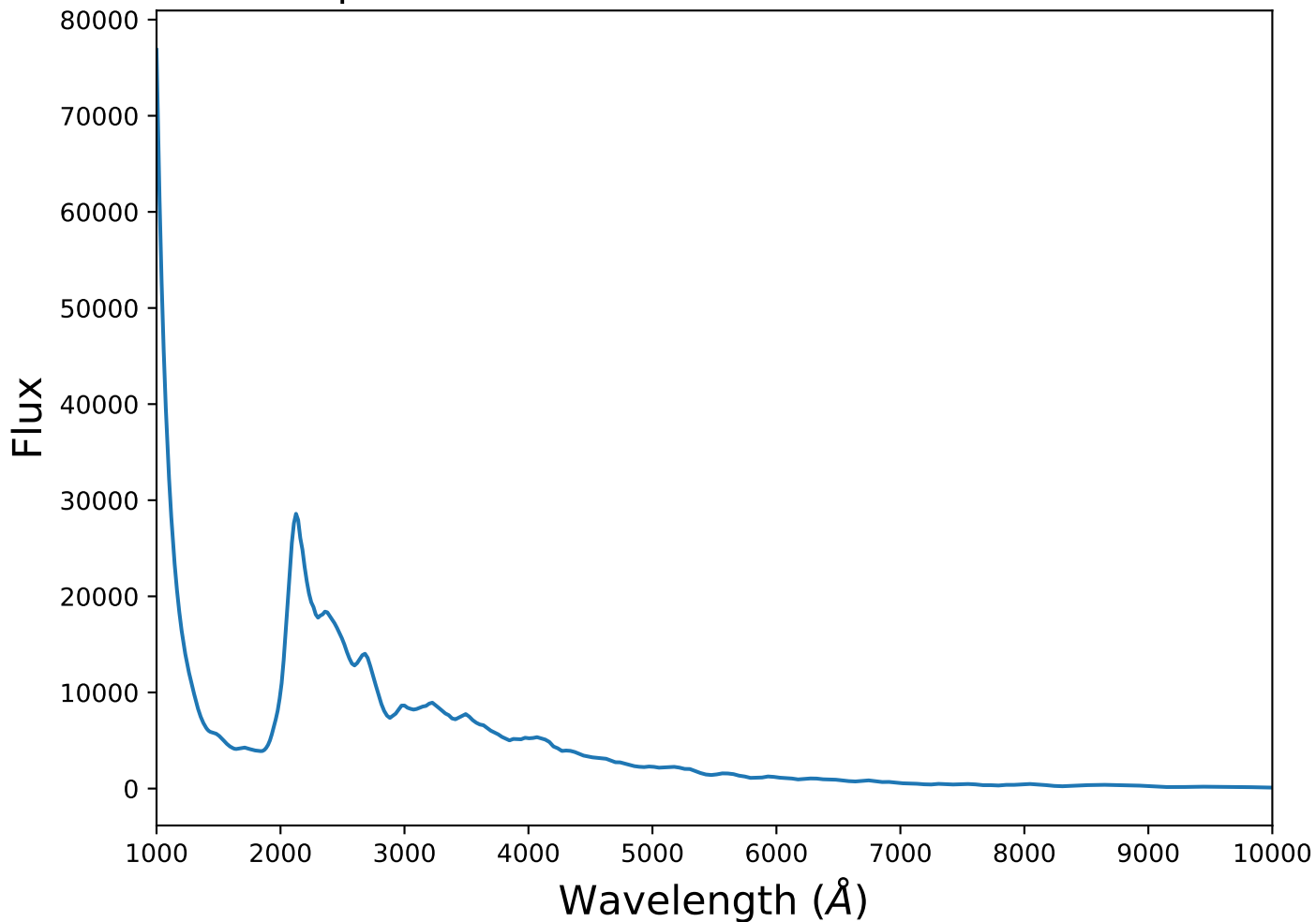
Spectrum 6 for transient SNIa at z=0.47
